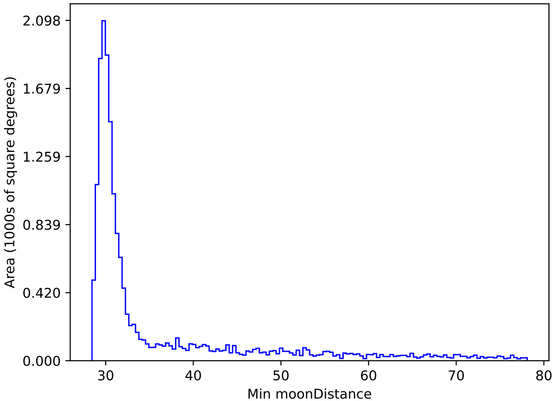
too_ignore_10_4v3.4_10yrs WFD i band: Min moonDistance
