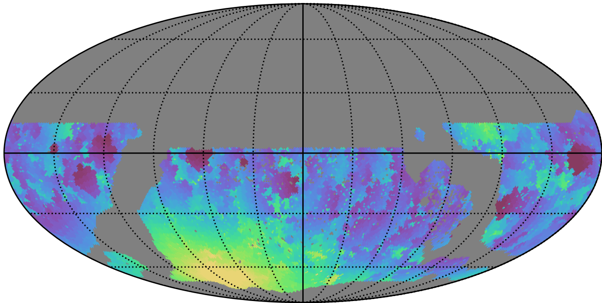
too_ignore_10_4v3.4_10yrs WFD g band: Min moonDistance
