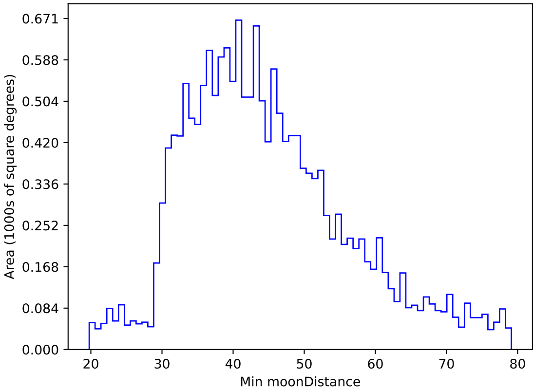
too_ignore_10_4v3.4_10yrs WFD g band: Min moonDistance
