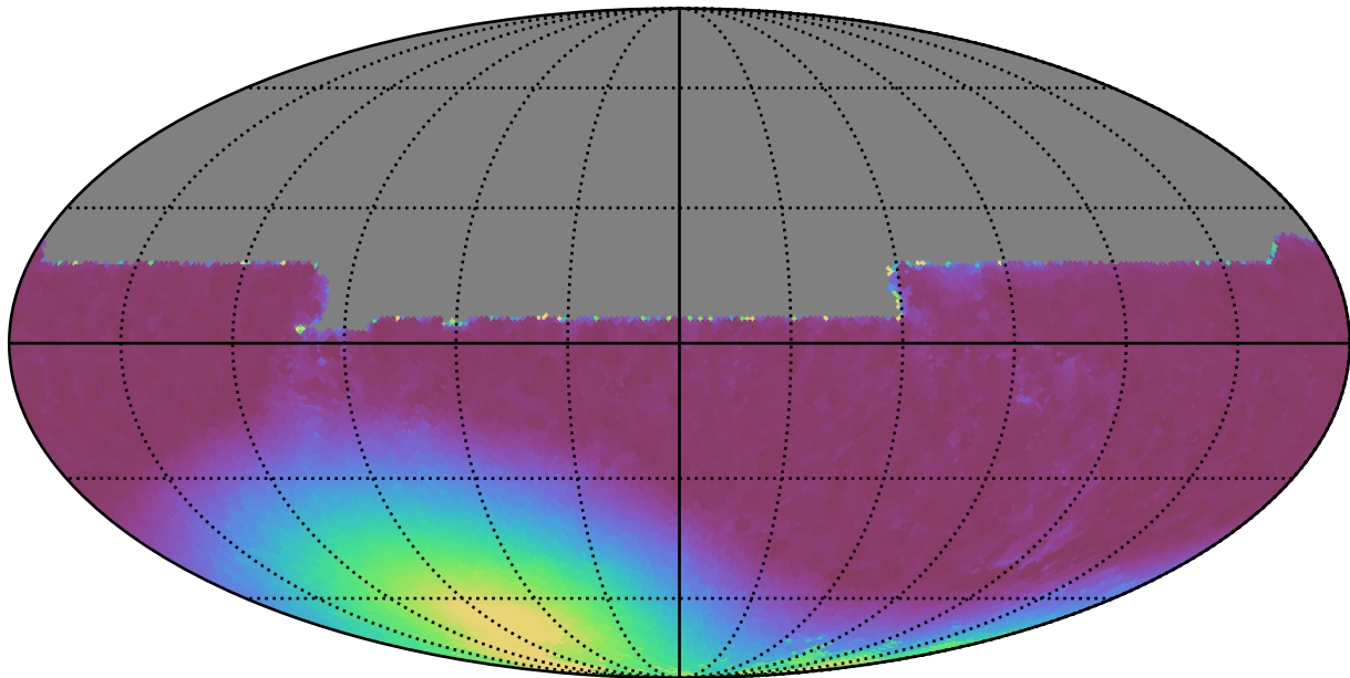
too_ignore_10_4v3.4_10yrs All sky y band: Min moonDistance
