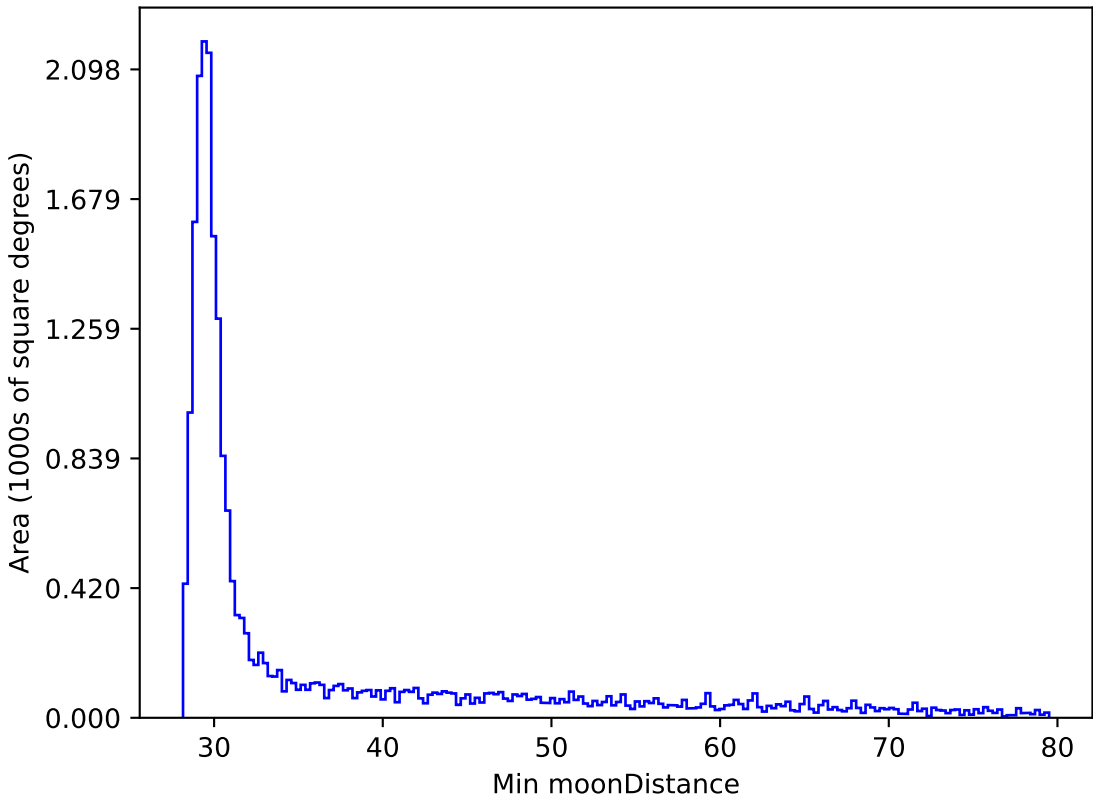
too_ignore_10_4v3.4_10yrs All sky y band: Min moonDistance
