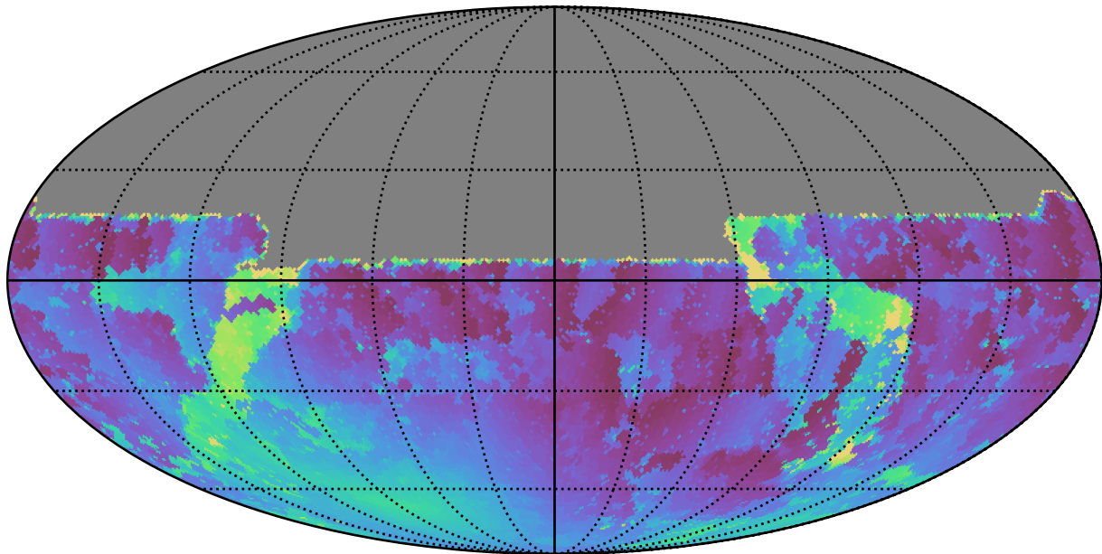
too_ignore_10_4v3.4_10yrs All sky u band: Min moonDistance
