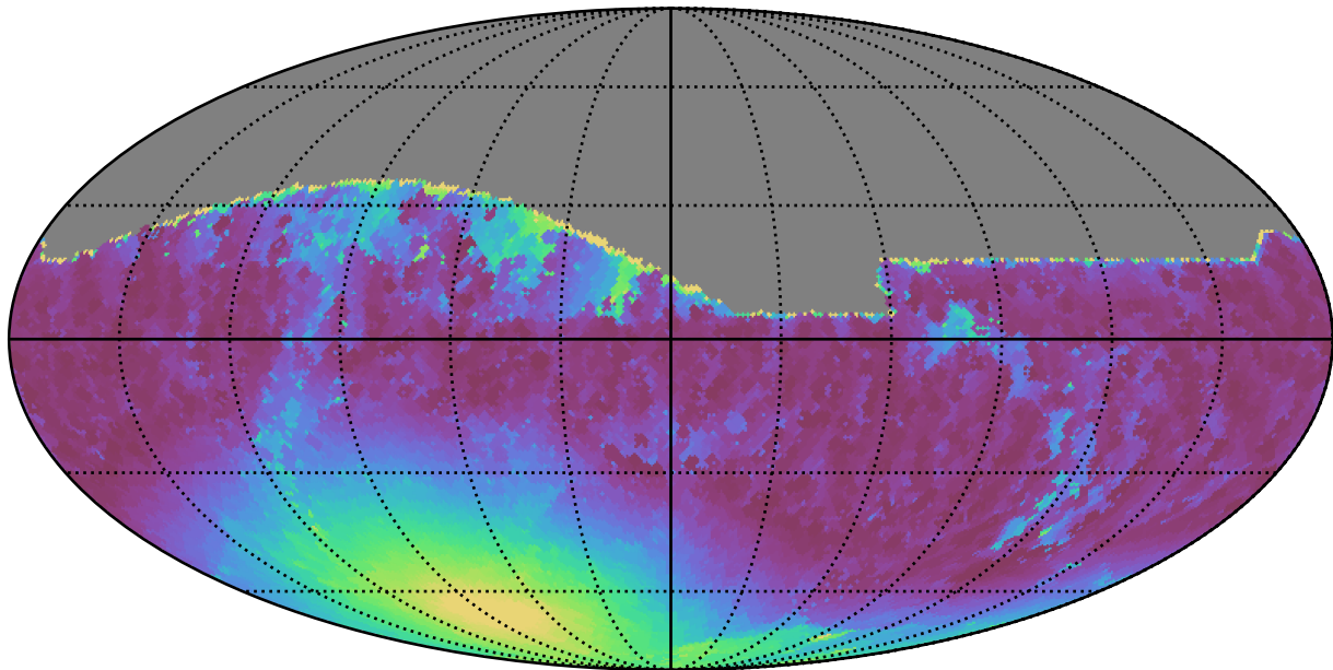
too_ignore_10_4v3.4_10yrs All sky r band: Min moonDistance
