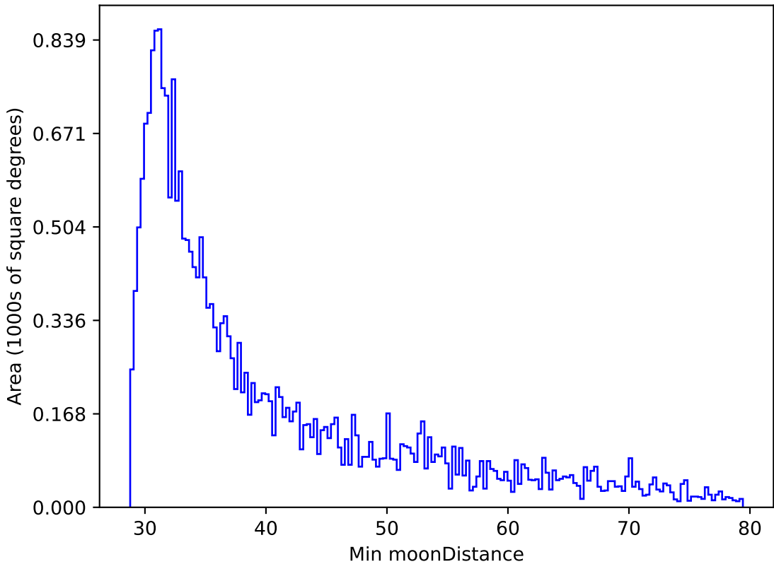
too_ignore_10_4v3.4_10yrs All sky r band: Min moonDistance
