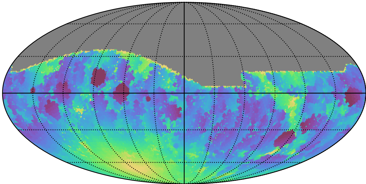
too_ignore_10_4v3.4_10yrs All sky g band: Min moonDistance
