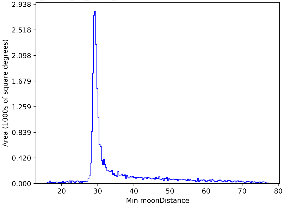
too_ignore_10_4v3.4_10yrs All sky all bands: Min moonDistance
