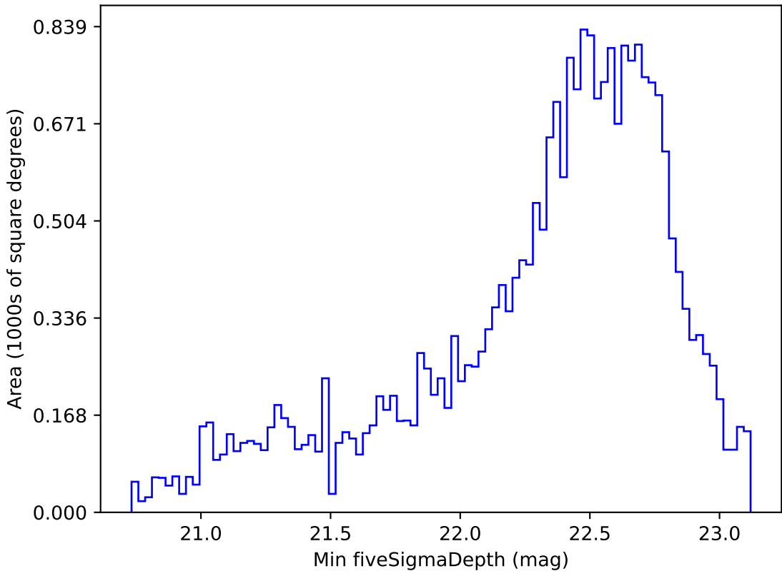
too_ignore_10_4v3.4_10yrs Yr 1 z band: Min fiveSigmaDepth
