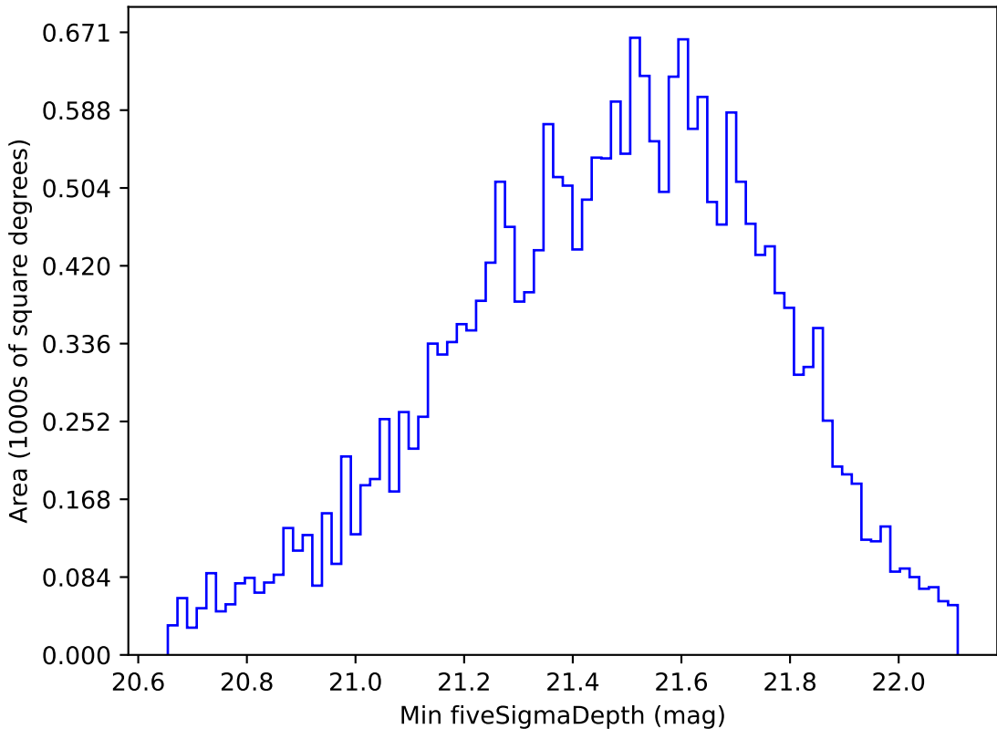
too_ignore_10_4v3.4_10yrs Yr 1 y band: Min fiveSigmaDepth
