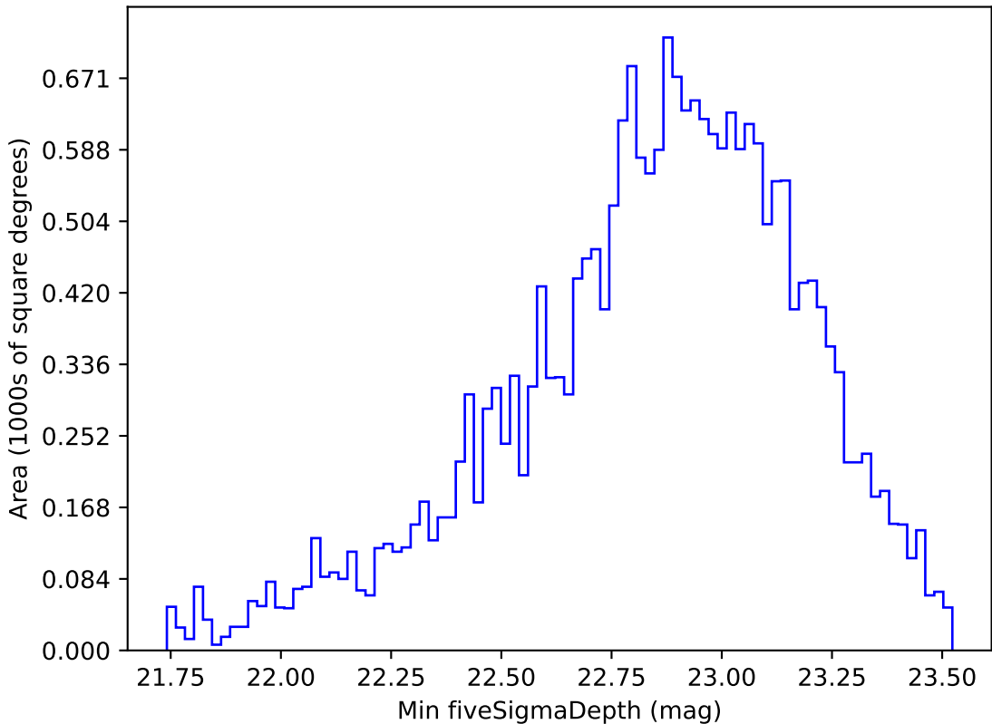
too_ignore_10_4v3.4_10yrs Yr 1 u band: Min fiveSigmaDepth
