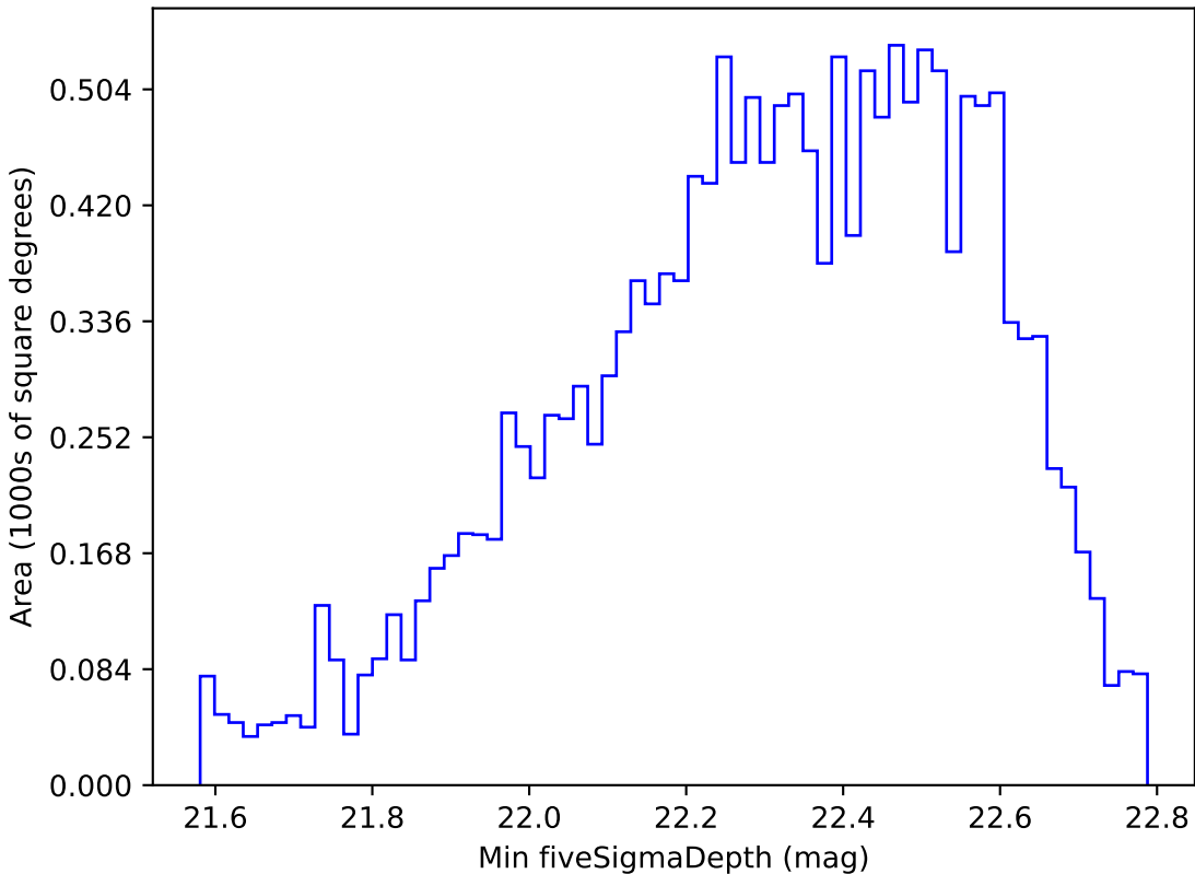
too_ignore_10_4v3.4_10yrs WFD u band: Min fiveSigmaDepth
