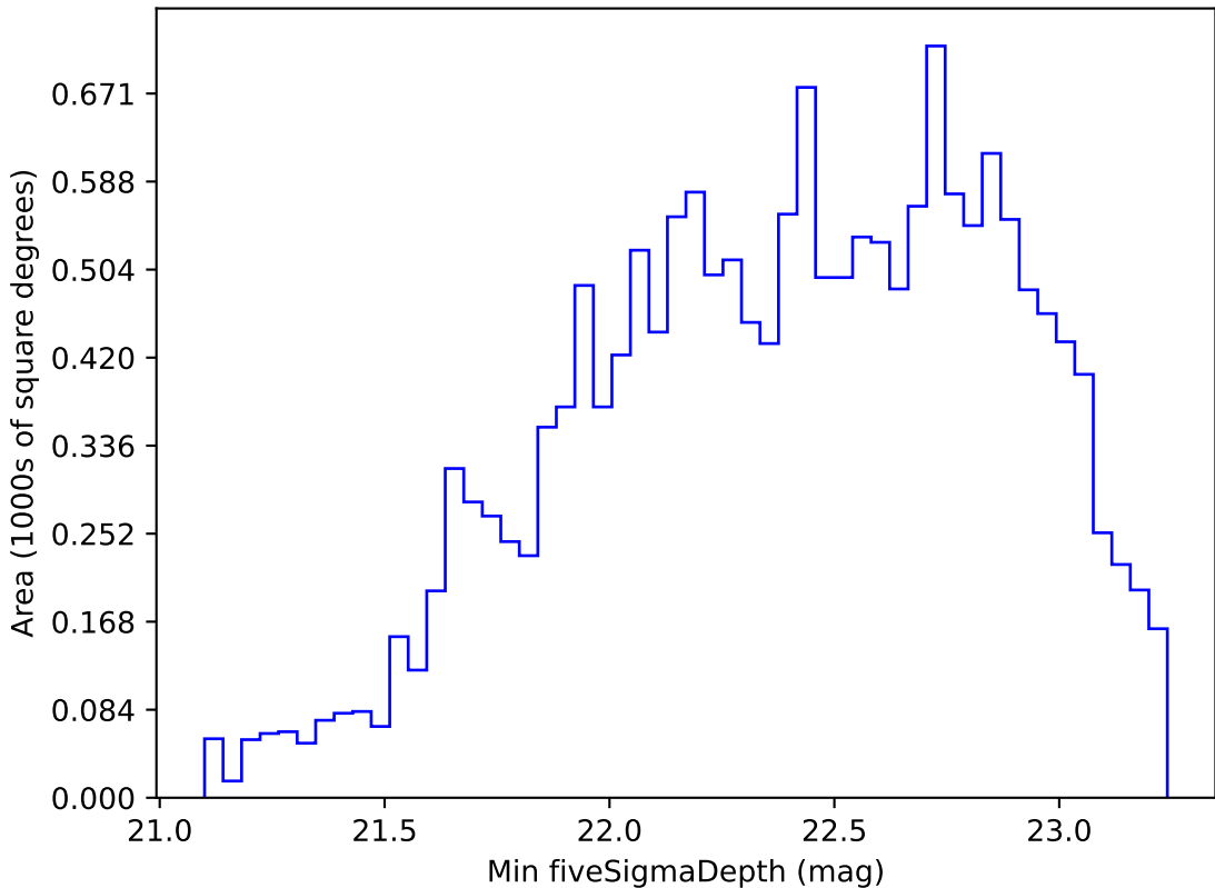
too_ignore_10_4v3.4_10yrs WFD r band: Min fiveSigmaDepth
