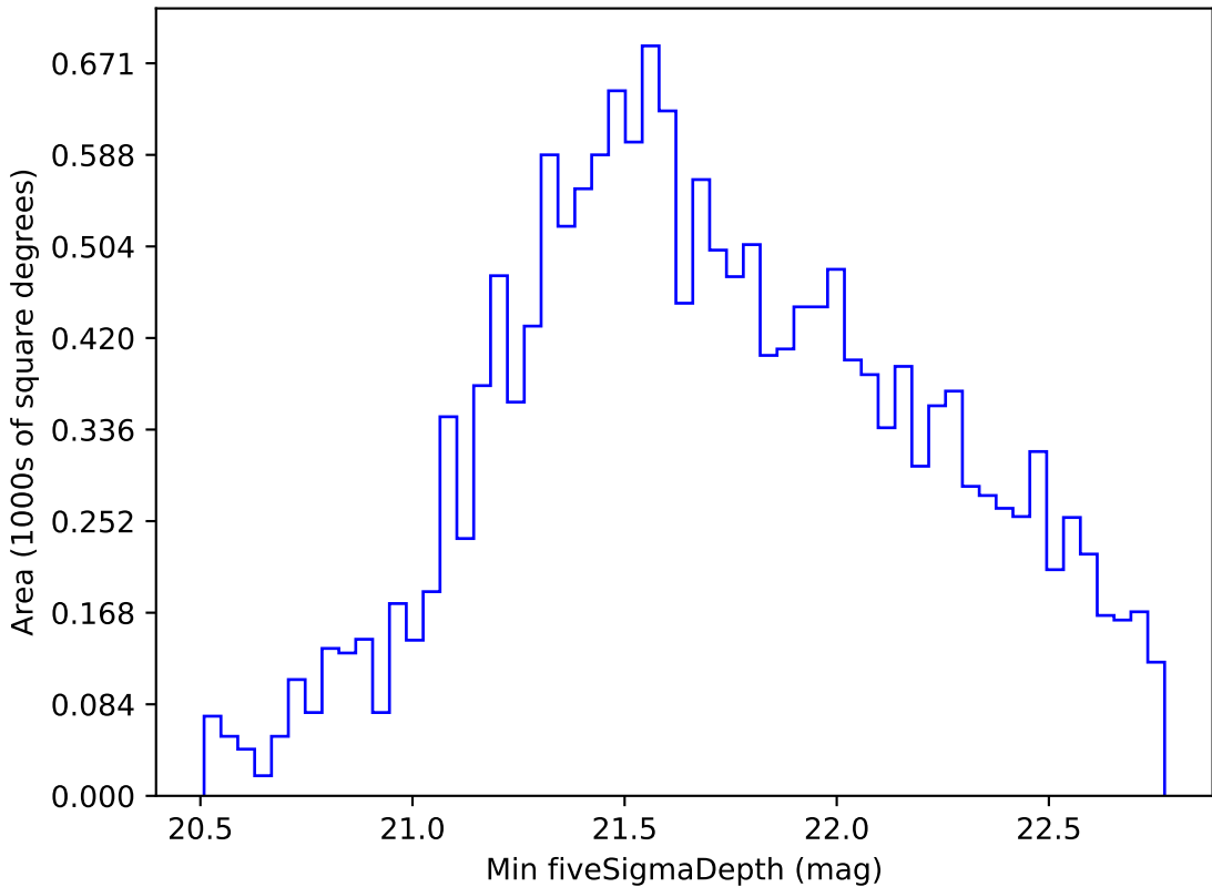
too_ignore_10_4v3.4_10yrs WFD i band: Min fiveSigmaDepth
