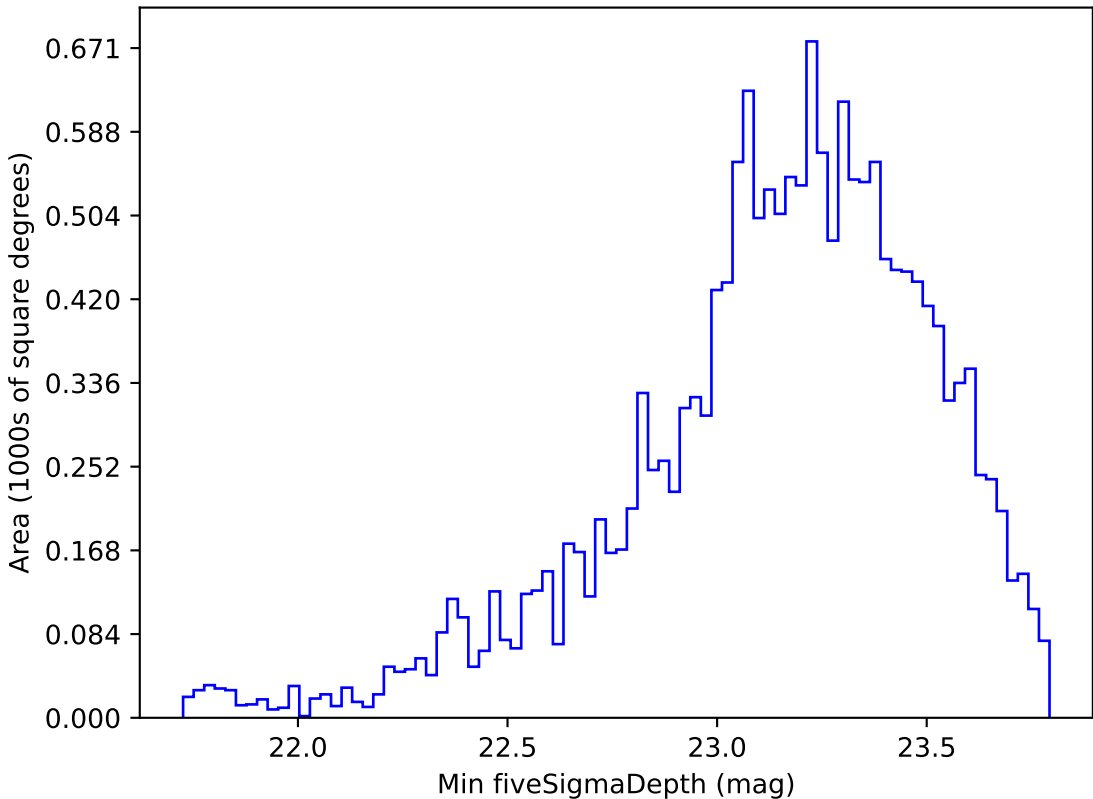
too_ignore_10_4v3.4_10yrs WFD g band: Min fiveSigmaDepth
