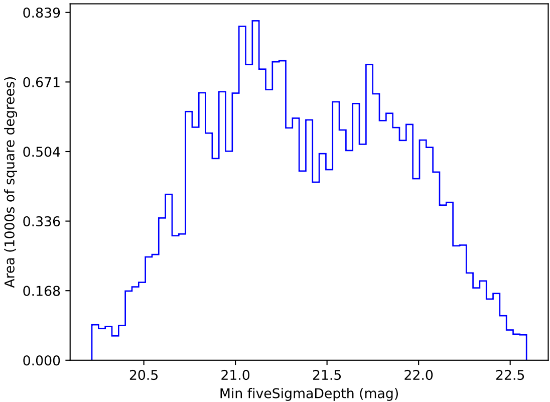
too_ignore_10_4v3.4_10yrs All sky z band: Min fiveSigmaDepth
