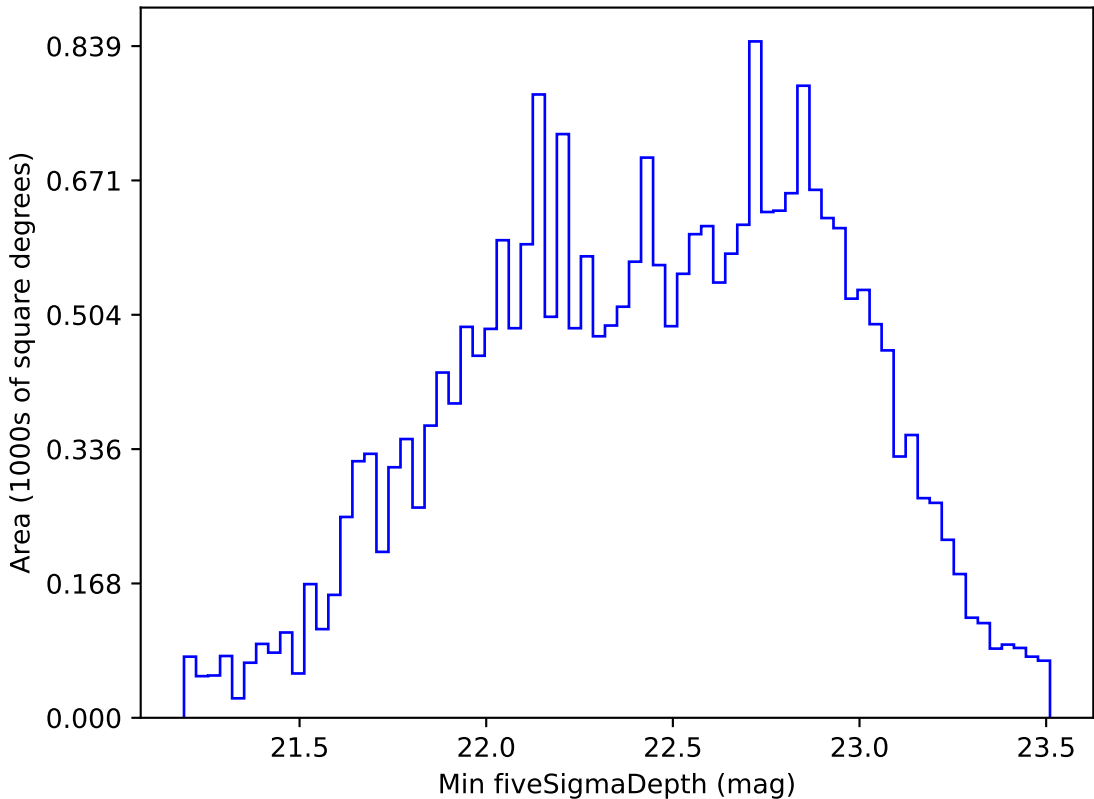
too_ignore_10_4v3.4_10yrs All sky r band: Min fiveSigmaDepth
