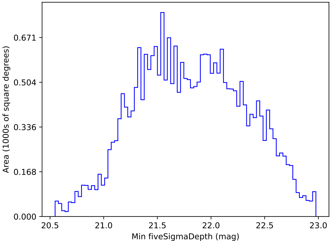
too_ignore_10_4v3.4_10yrs All sky i band: Min fiveSigmaDepth
