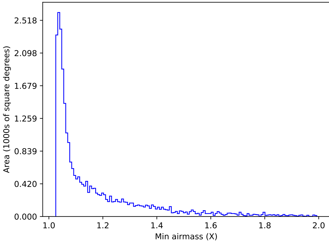
too_ignore_10_4v3.4_10yrs Yr 1 z band: Min airmass
