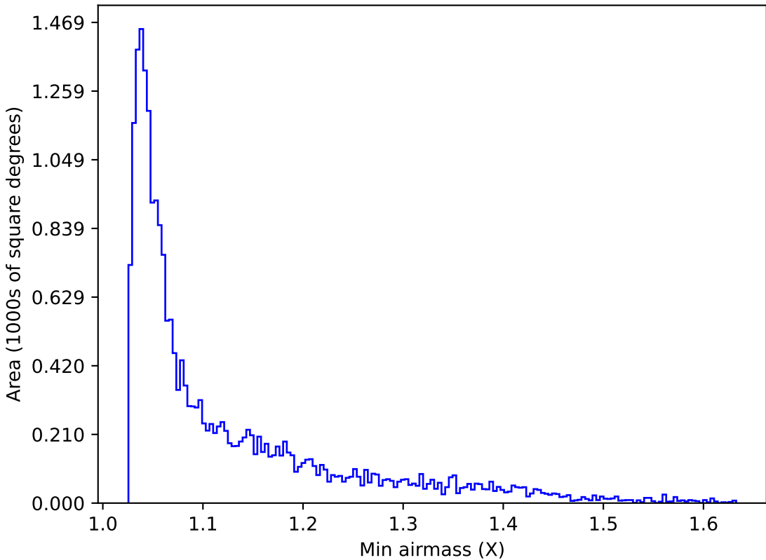
too_ignore_10_4v3.4_10yrs Yr 1 y band: Min airmass
