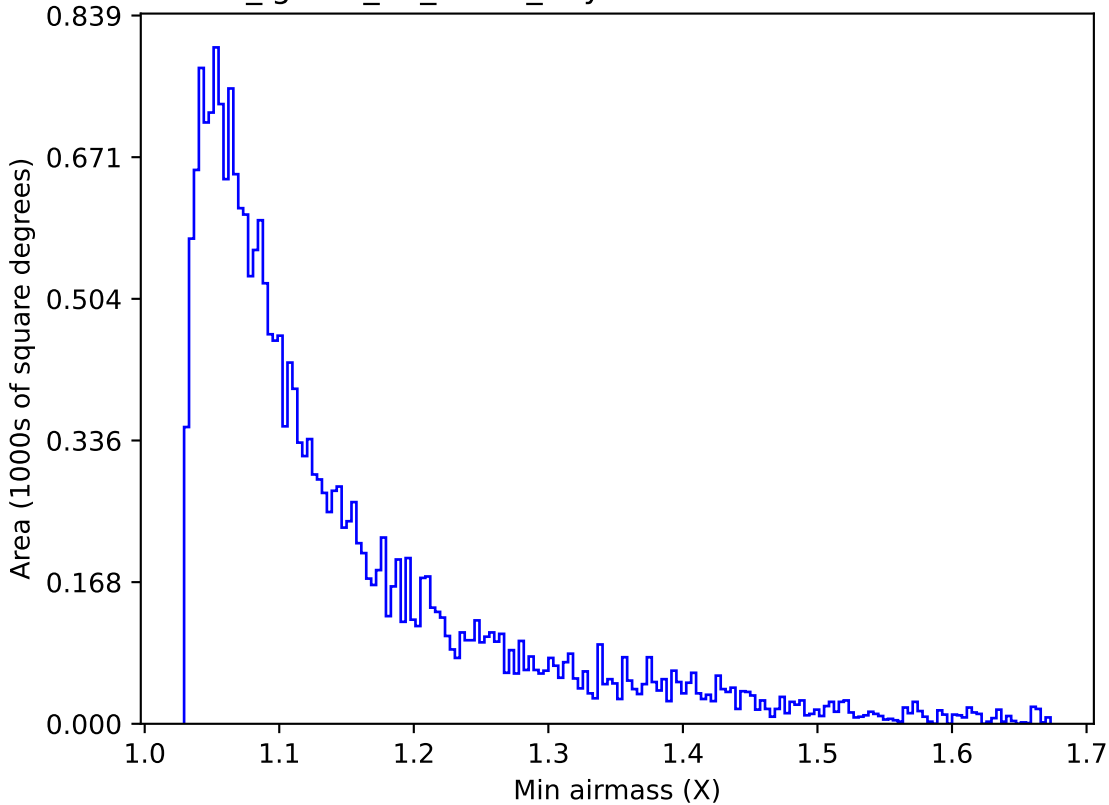
too_ignore_10_4v3.4_10yrs Yr 1 u band: Min airmass
