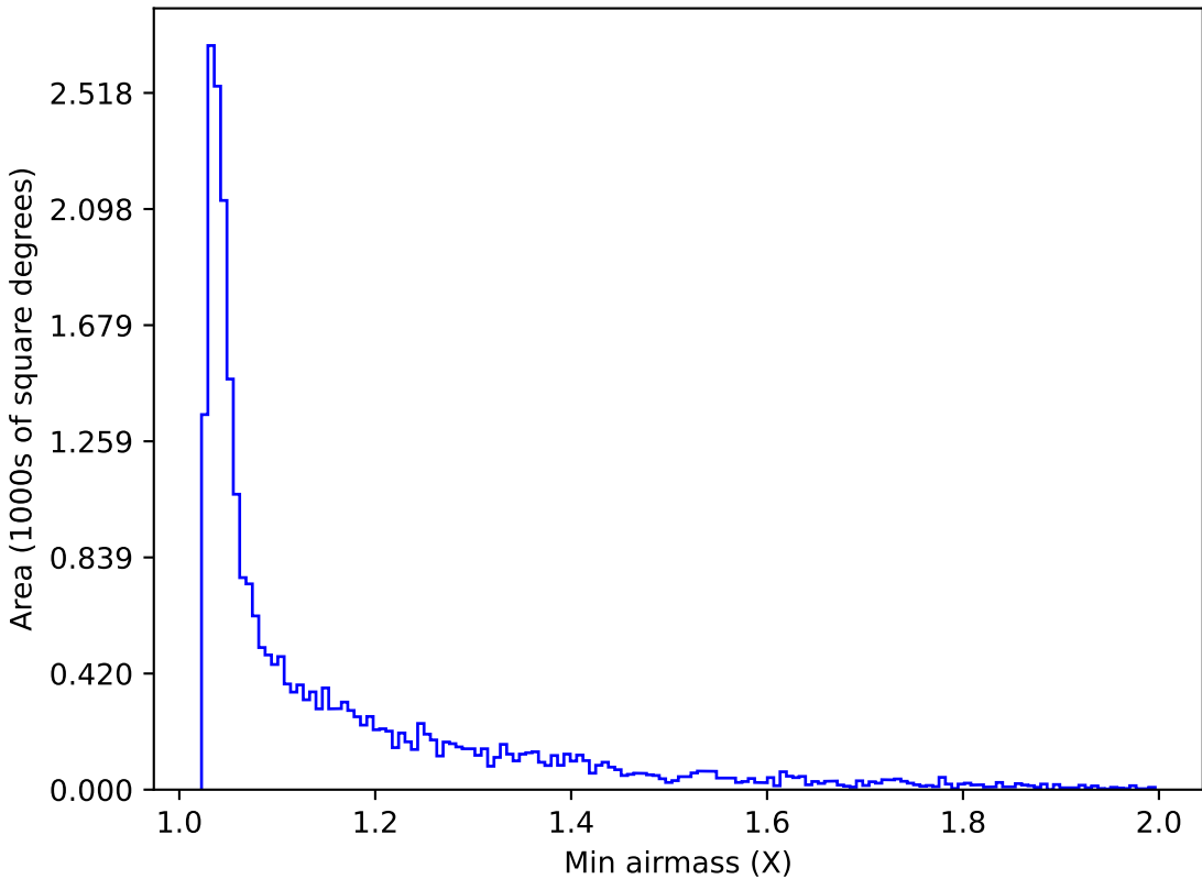
too_ignore_10_4v3.4_10yrs Yr 1 r band: Min airmass
