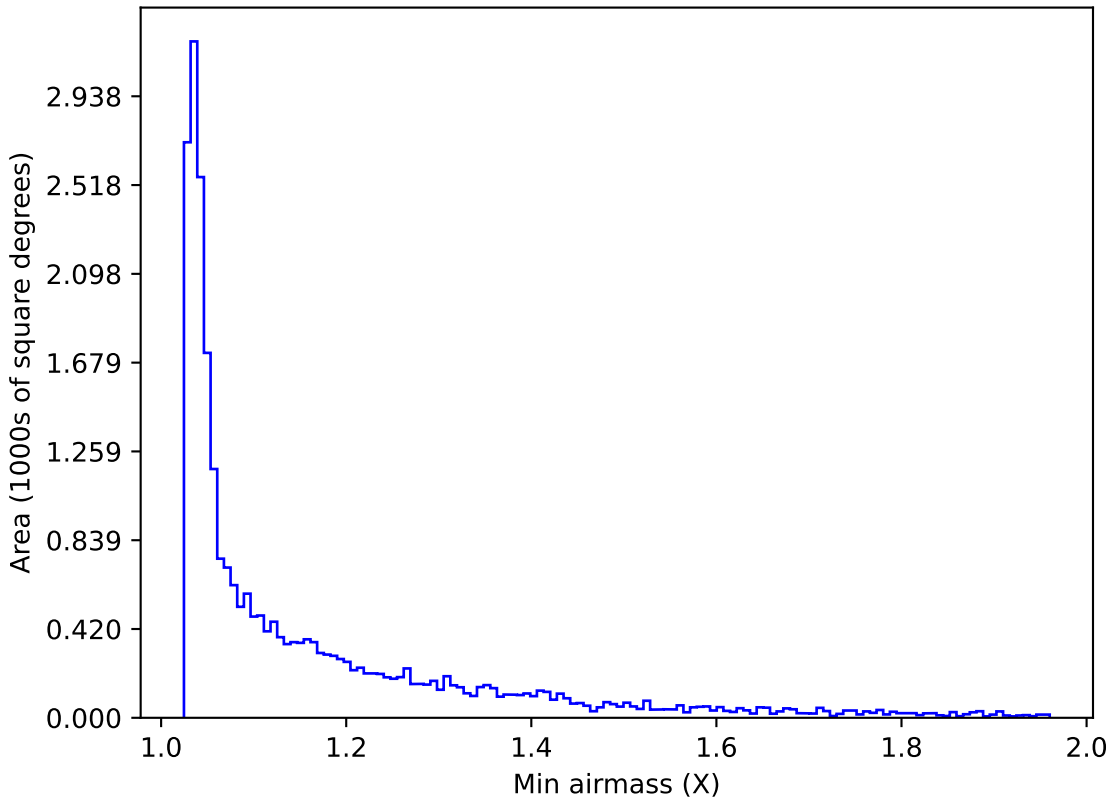
too_ignore_10_4v3.4_10yrs Yr 1 i band: Min airmass
