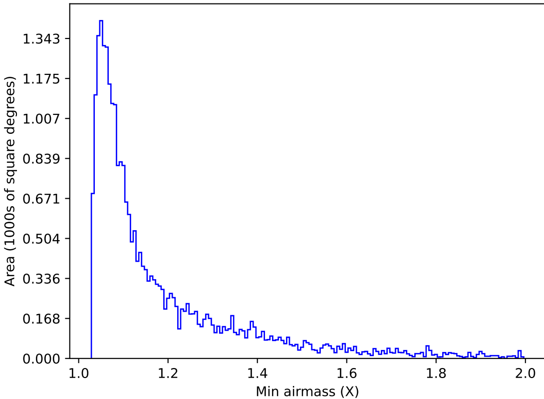
too_ignore_10_4v3.4_10yrs Yr 1 g band: Min airmass
