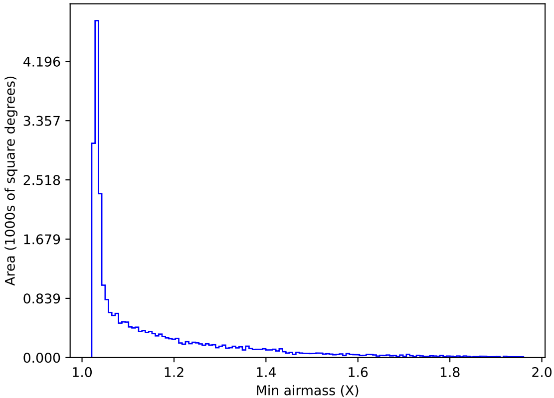
too_ignore_10_4v3.4_10yrs Yr 1 all bands: Min airmass
