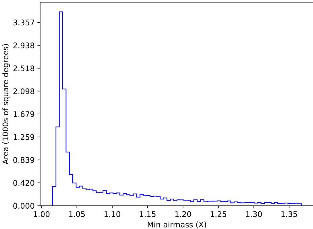
too_ignore_10_4v3.4_10yrs WFD z band: Min airmass
