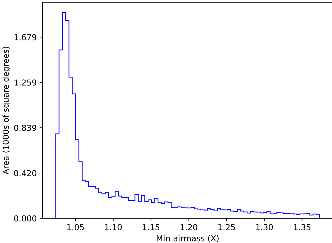
too_ignore_10_4v3.4_10yrs WFD u band: Min airmass
