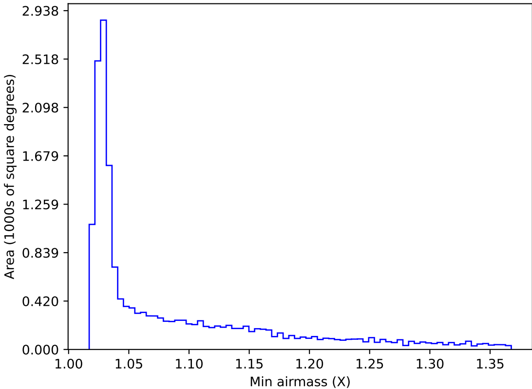
too_ignore_10_4v3.4_10yrs WFD r band: Min airmass
