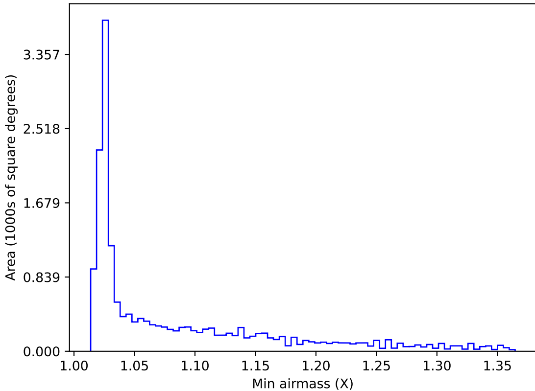
too_ignore_10_4v3.4_10yrs WFD all bands: Min airmass
