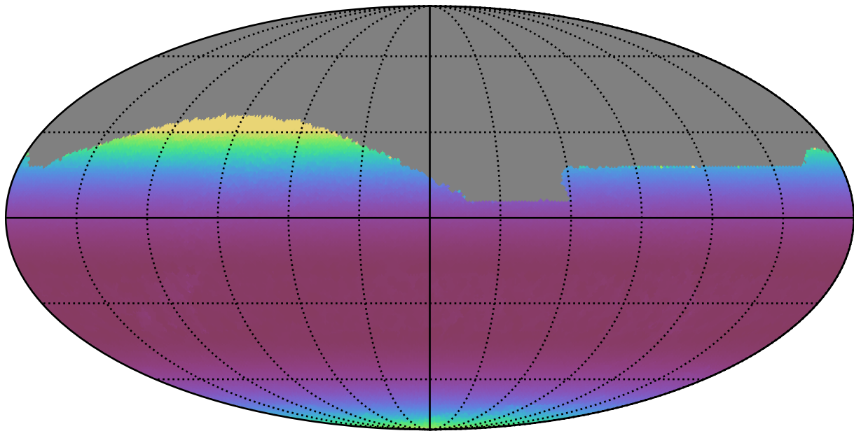
too_ignore_10_4v3.4_10yrs All sky z band: Min airmass
