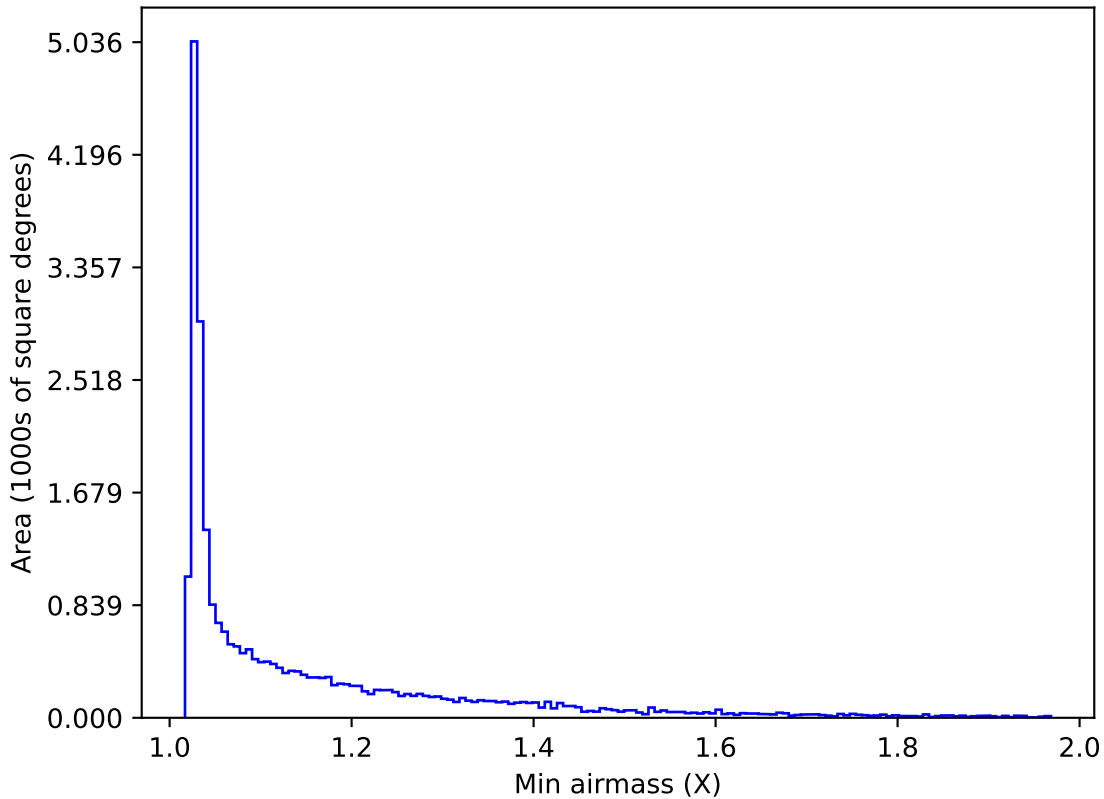
too_ignore_10_4v3.4_10yrs All sky z band: Min airmass
