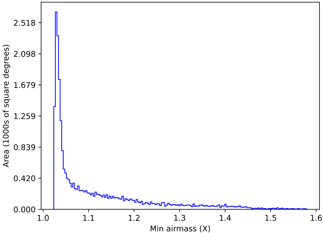
too_ignore_10_4v3.4_10yrs All sky y band: Min airmass
