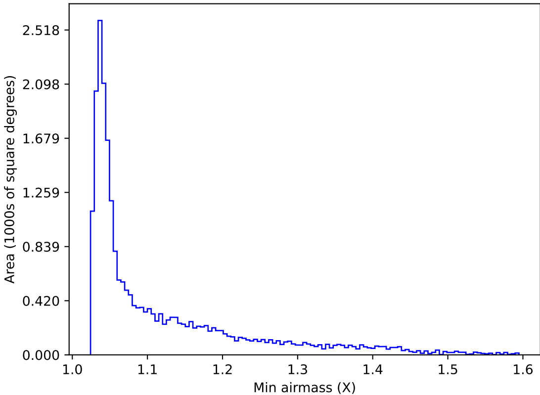
too_ignore_10_4v3.4_10yrs All sky u band: Min airmass
