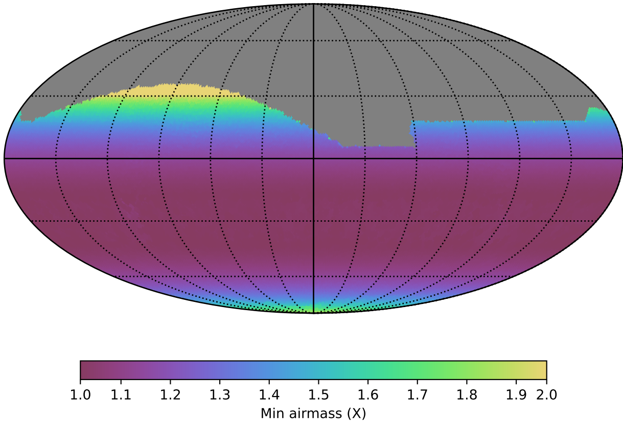
too_ignore_10_4v3.4_10yrs All sky r band: Min airmass
