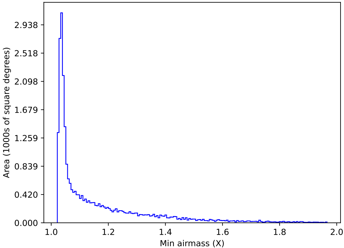
too_ignore_10_4v3.4_10yrs All sky g band: Min airmass
