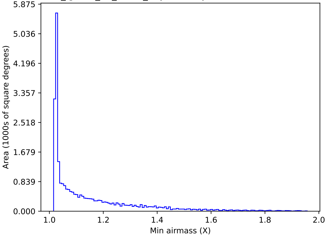
too_ignore_10_4v3.4_10yrs All sky all bands: Min airmass
