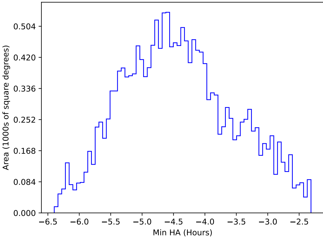
too_ignore_10_4v3.4_10yrs WFD r band: Min HA
