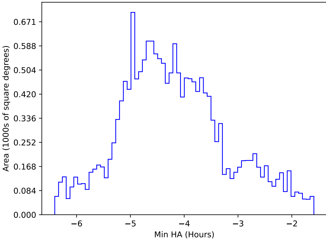
too_ignore_10_4v3.4_10yrs WFD g band: Min HA
