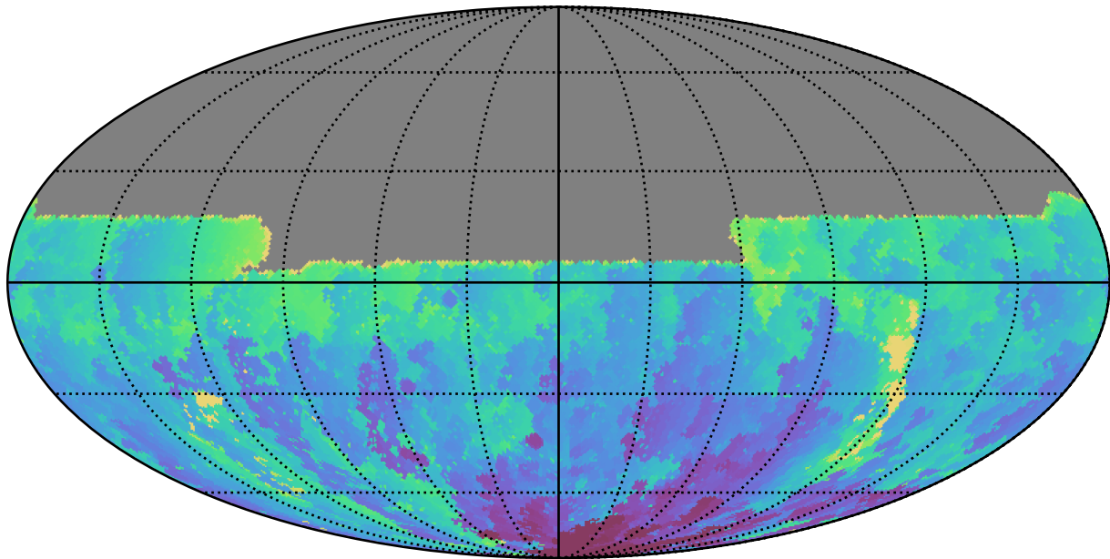
too_ignore_10_4v3.4_10yrs All sky u band: Min HA
