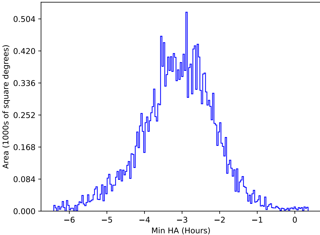
too_ignore_10_4v3.4_10yrs All sky u band: Min HA
