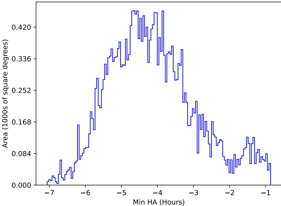
too_ignore_10_4v3.4_10yrs All sky r band: Min HA
