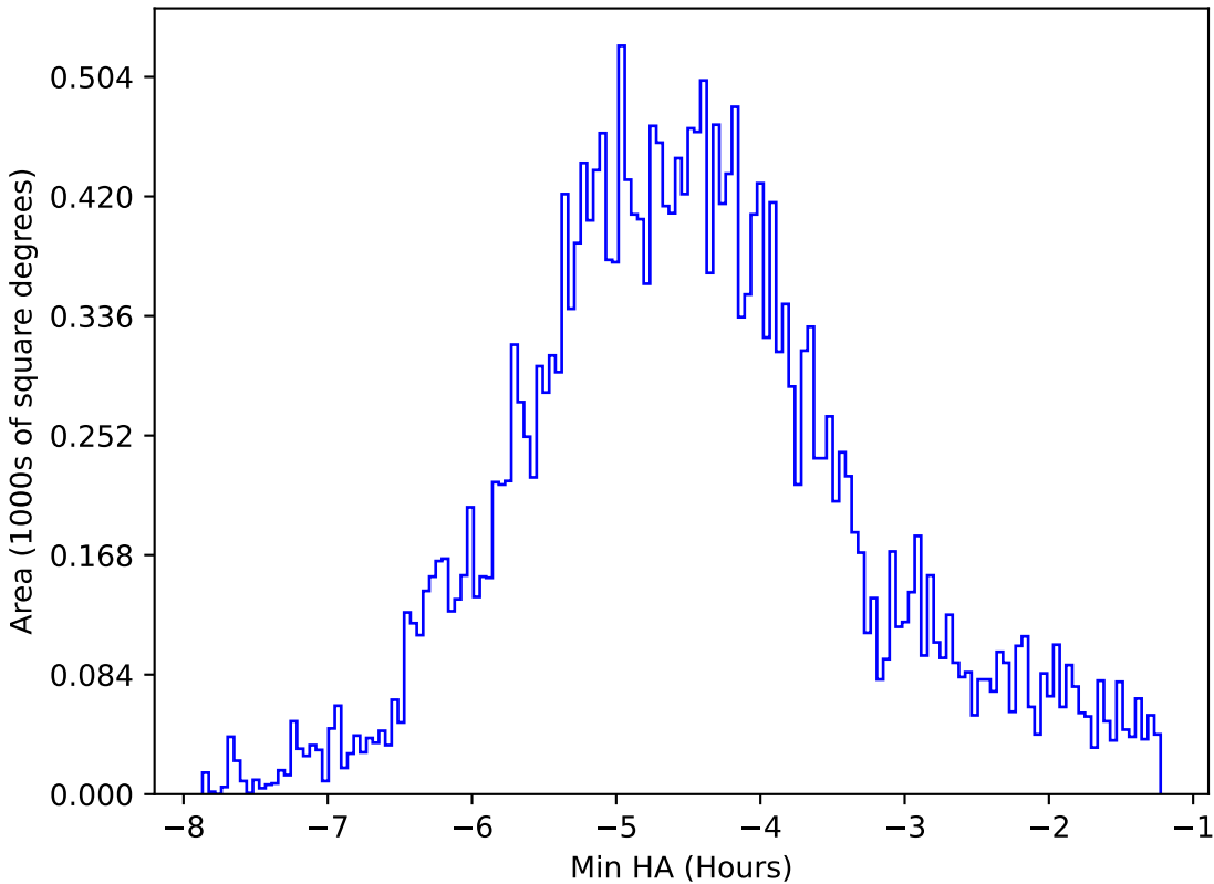
too_ignore_10_4v3.4_10yrs All sky all bands: Min HA
