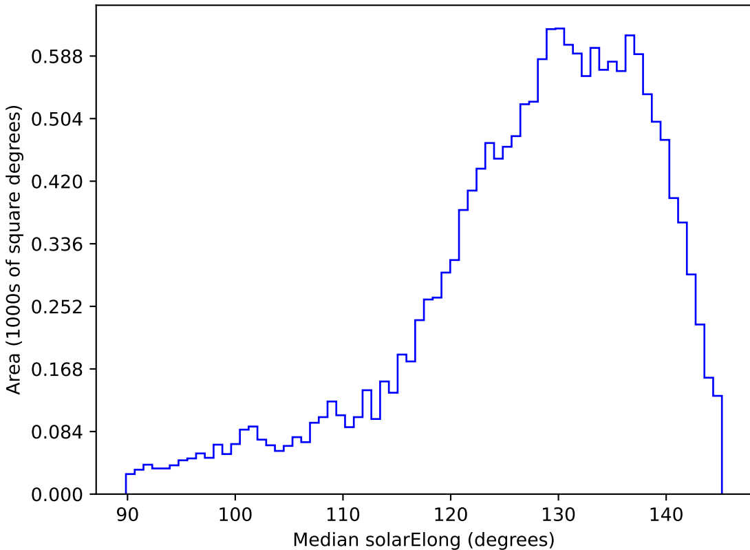
too_ignore_10_4v3.4_10yrs WFD z band: Median solarElong
