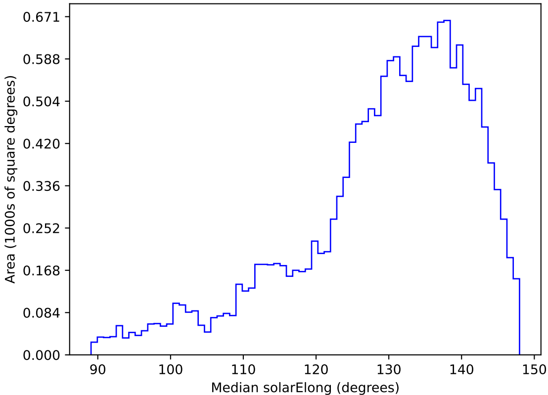
too_ignore_10_4v3.4_10yrs WFD y band: Median solarElong
