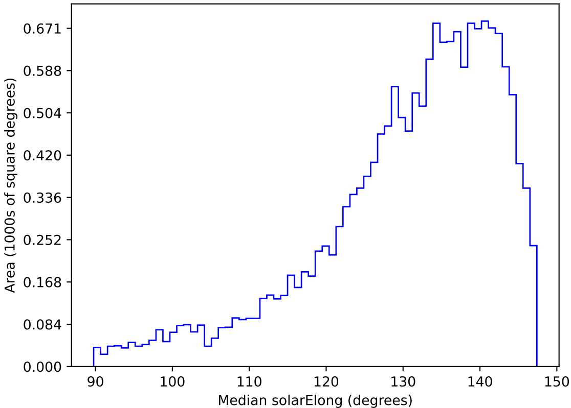
too_ignore_10_4v3.4_10yrs WFD r band: Median solarElong
