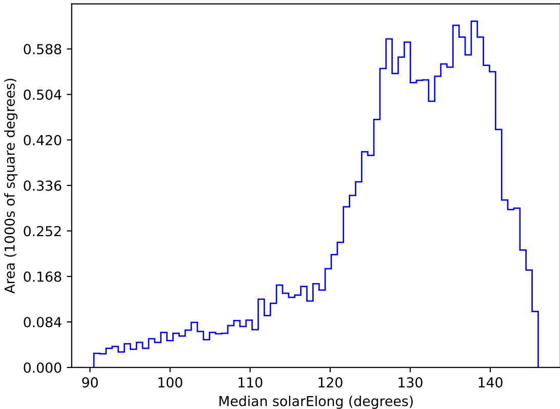
too_ignore_10_4v3.4_10yrs WFD i band: Median solarElong
