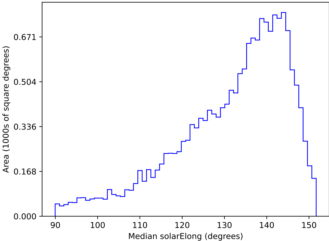
too_ignore_10_4v3.4_10yrs WFD g band: Median solarElong
