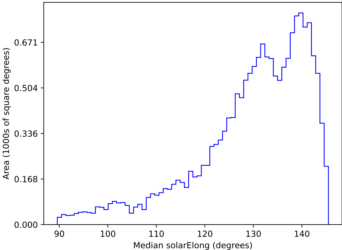
too_ignore_10_4v3.4_10yrs WFD all bands: Median solarElong
